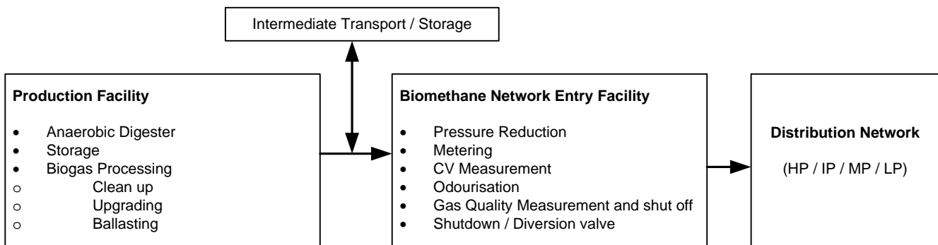
Figure 1 - Biomethane Supply Chain & Component Groups
