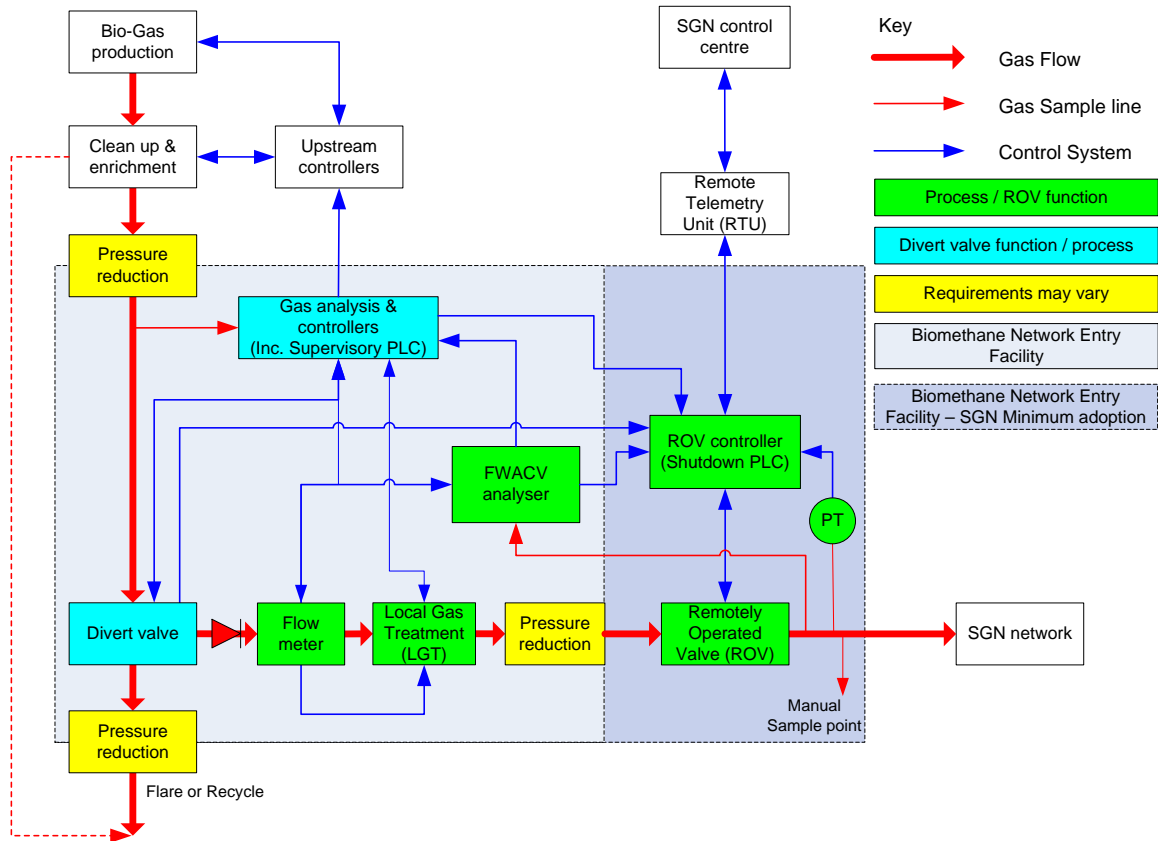
Figure 2 – BNEF Functional Block Diagram
